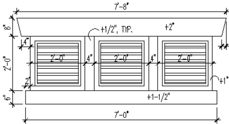
FOAM DETAIL
