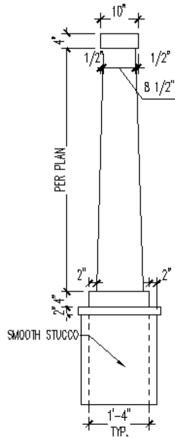
COLUMN DETAIL
