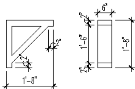
CRAFTSMAN BRACKET
