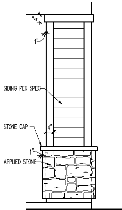
COLUMN DETAIL
