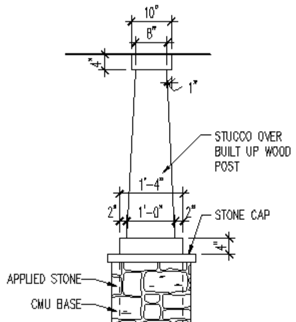
COLUMN DETAIL
