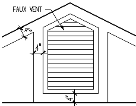
VENT DETAIL
